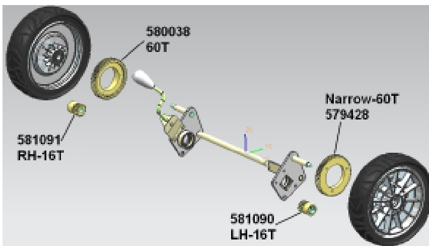
Old Driving Gears configuration
