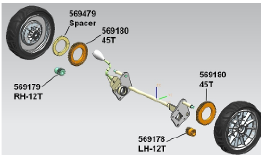
New Driving Gears configuration
